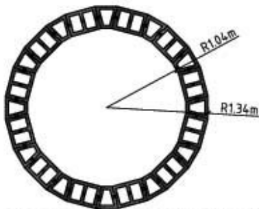
C30-CORNER BLOCK + B1-FULL BLOCK 1:50
