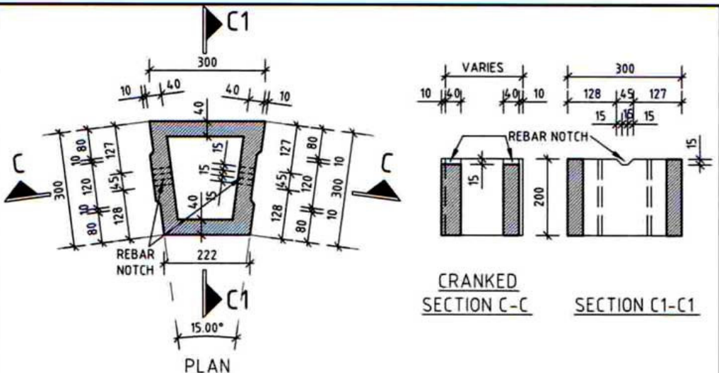
15° CORNER BLOCK - BLOCK C15 1:10
