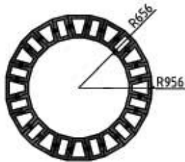
C30-CORNER BLOCK + B2-HALF BLOCK 1:50
