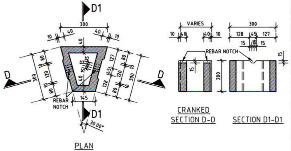
30° CORNER BLOCK - BLOCK C30 1:10
